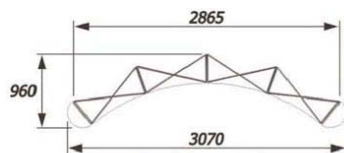
3 x 4 - Curved
