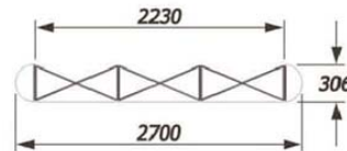
3 x 3 - Straight
