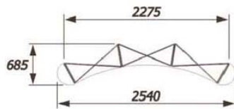
3 x 3 - Curved
